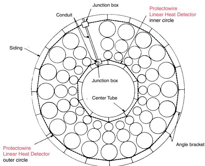
Figure 6A Base view horizontal section
