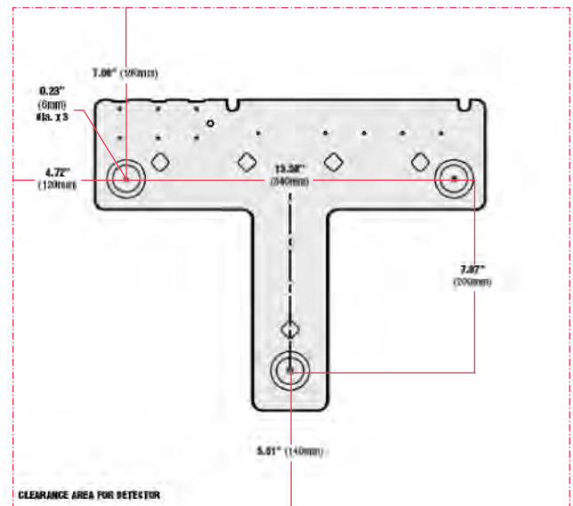
Stratos Mounting Plate Dimensions
